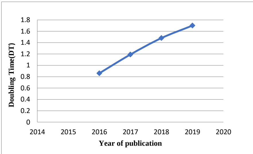
Figure 2: Doubling time of publications
